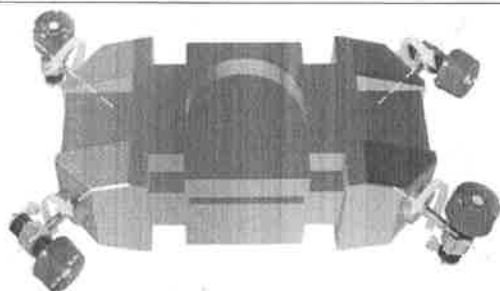
Fig 2. Conceptual design of the proposed vehicle system with four tilting thrusters The proposed manipulator arm will have at least 3 DOF in order to provide dexterity and redundancy. The proposed preliminary design consists of three rotary joints followed as an articulated robot. The conceptual design of the vehicle manipulator system is presented in Fig. 3. The manipulator system will also be sealed and depth rated with similar specifications as that of the vehicle hull.
